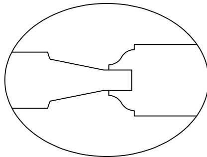
BELMONT PANEL OGEE STICKING
