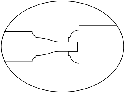
LANDSCAPE PANEL STANDARD STICKING
